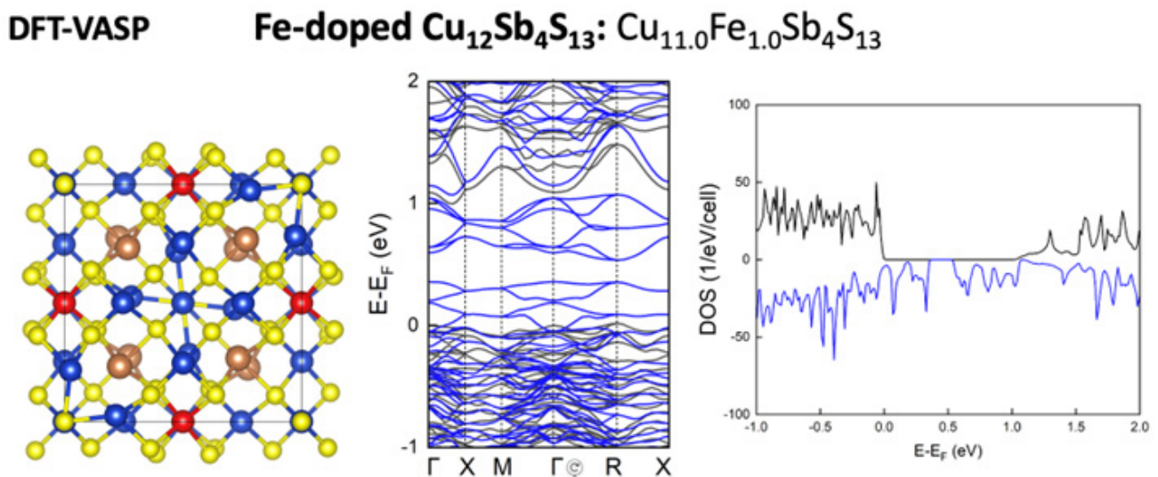
Figure 3 - Iron introduces new electronic states in the band gap of tetrahedrite. Relaxed atomic structure, electronic band structure, and density of states of \text{Cu}_{11.0}\text{Fe}_{1.0}\text{Sb}_4\text{S}_{13} . The blue, yellow, orange, and red spheres correspond to Cu, S, Sb and Fe atoms, respectively.
