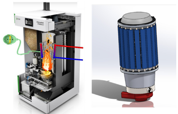
Figure 21 -(Left) TEG systems integrated into commercial boilers for CHP systems; (Right) Cylindrical TEG systems.
